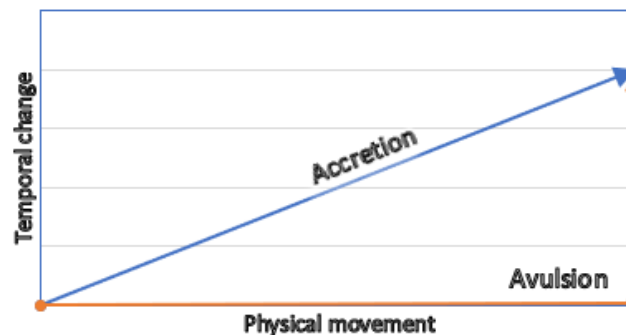
Figure 3: Accretion versus Avulsion by time and distance
