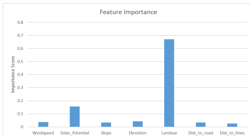
Figure 6: Feature Importance
