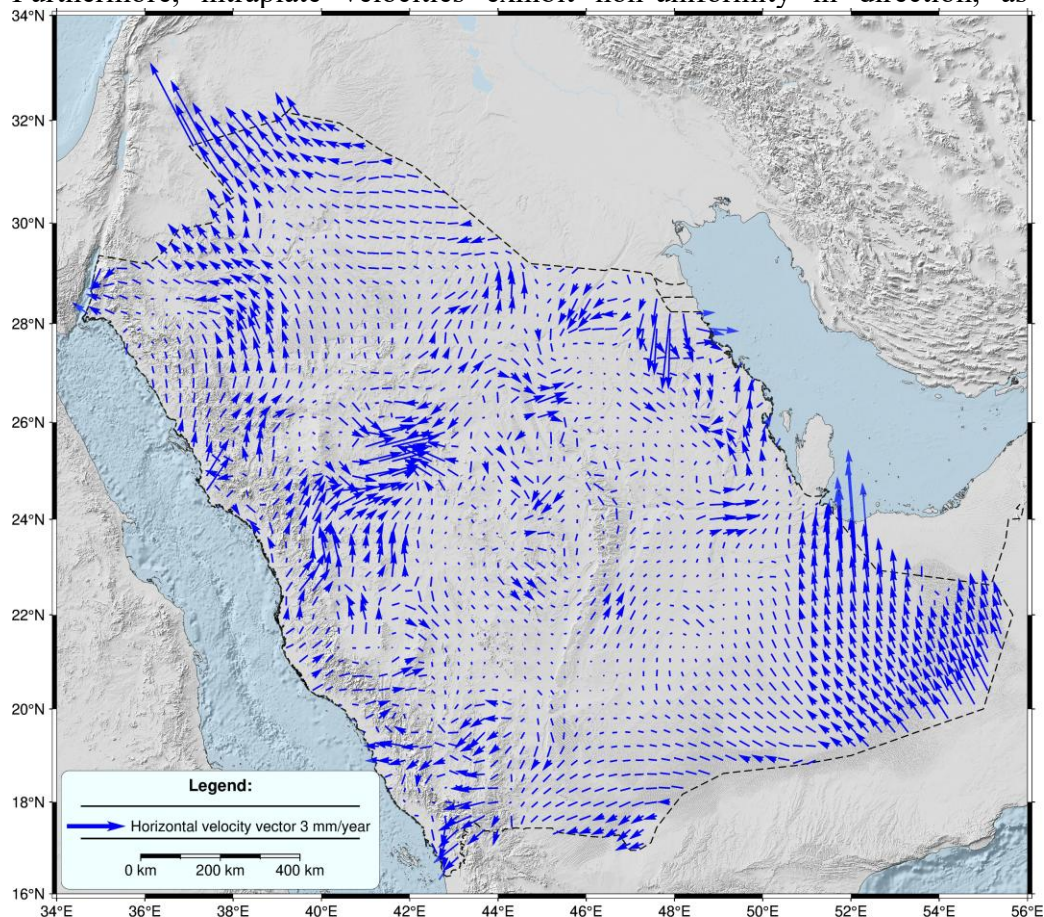
Figure 7. This spatial inhomogeneity introduces additional deleterious effects on positional accuracy. The magnitude of this impact can be estimated by calculating the intraplate offset the change in distance between two points resulting from their relative displacement.
