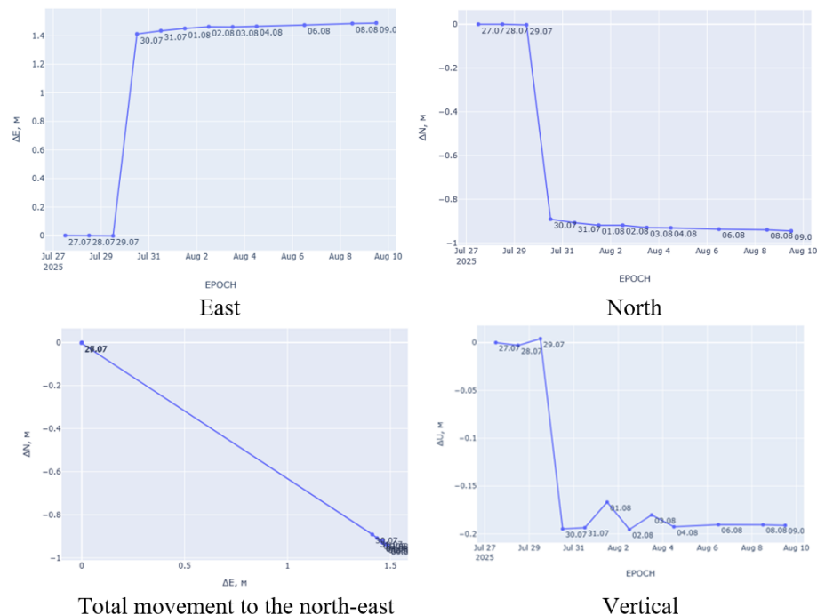
Figure 4. The results of processing the data of the SVK-1 point at the time of the earthquake
