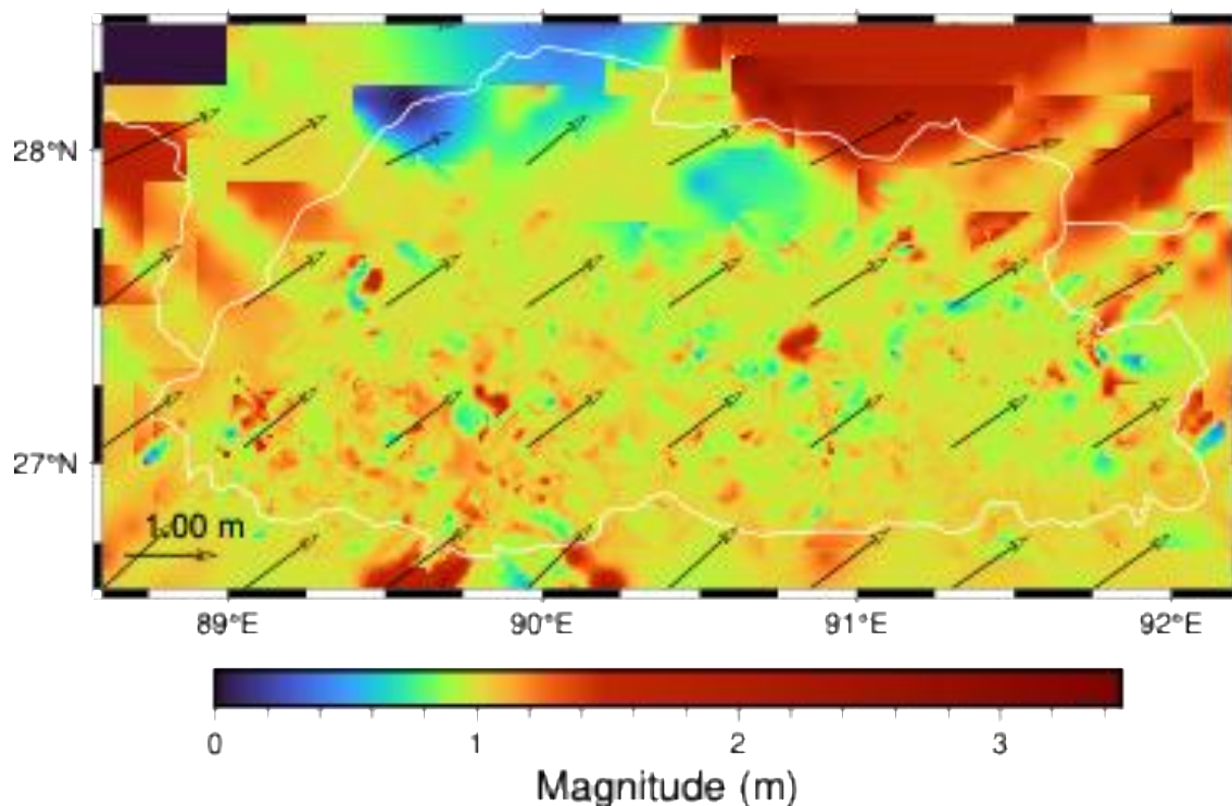
Figure 7: Final 10'' NTv2 horizontal-shift field (DrukRef03 → DrukRef23) over Bhutan.
