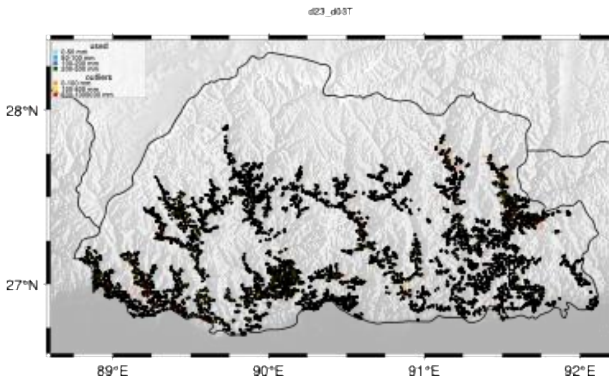
Figure 6: Residual classification of GNSS control points after iterative filtering. Colours indicate residual agnitude and exclusion status.
