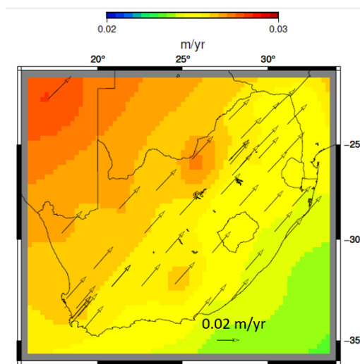
Figure 8 Velocity grid for South Africa. Colors show the magnitude of the combined e and u velocities in m. Areas outside the grid extents are shaded in grey. Velocity measurements used to constrain the grid are shown as vectors.
