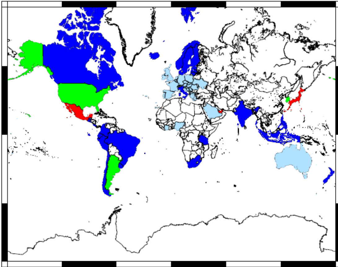
Figure 3 Map showing countries with Dynamic Datums. Countries in light blue model crustal motion using an Euler Pole. Countries in dark blue have a velocity grid. Countries in green use a full displacement model including a velocity model and earthquake grids and countries in red provide an online calculator, which we implement as a distortion grid.
