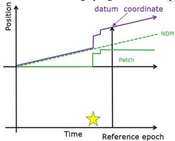
Figure 2 Schematic diagram of a dynamic datum. Dashed green line shows the secular velocity solid green line shows the co-seismic contribution to the displacement mode. The solid purple line shows the displacement model with both contributions combined.
