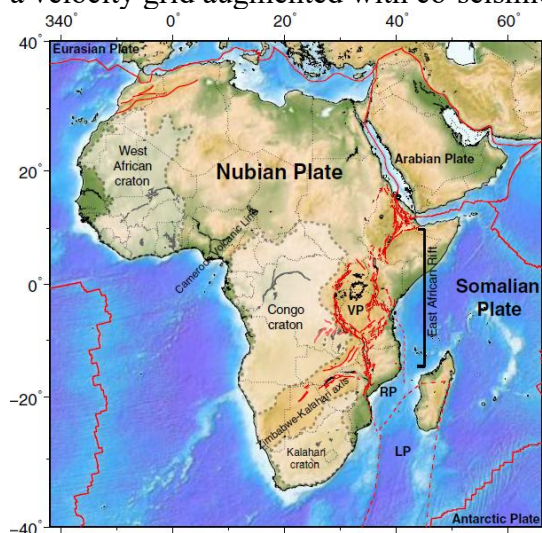
Figure 4 Tectonic environment of Africa from Saria et al (2013) VP refers to the Victoria micro plate and RP refers to the Rovuma micro plate.
