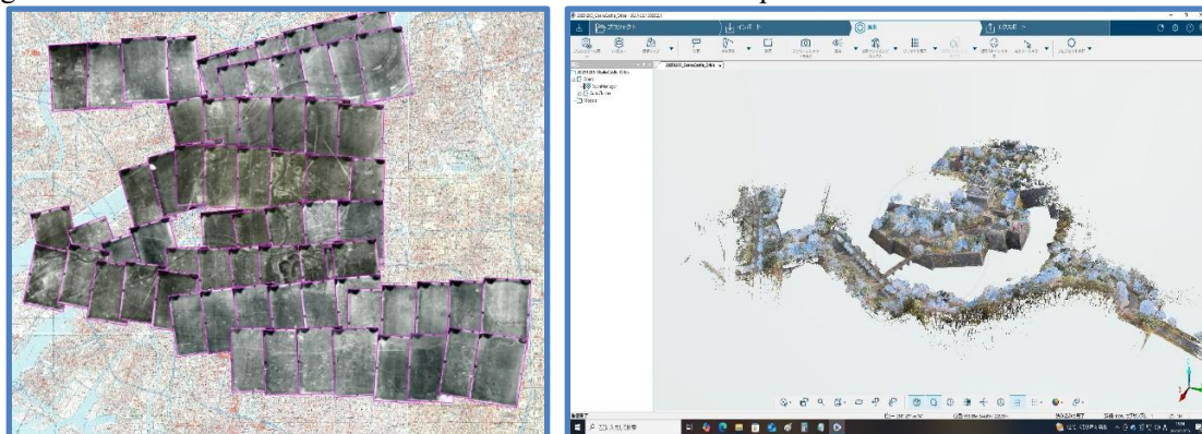
Figure 3-2-2 1928 ortho-mosaic photos : 2025 FARO 3D point cloud ( OsakaJyo park)
