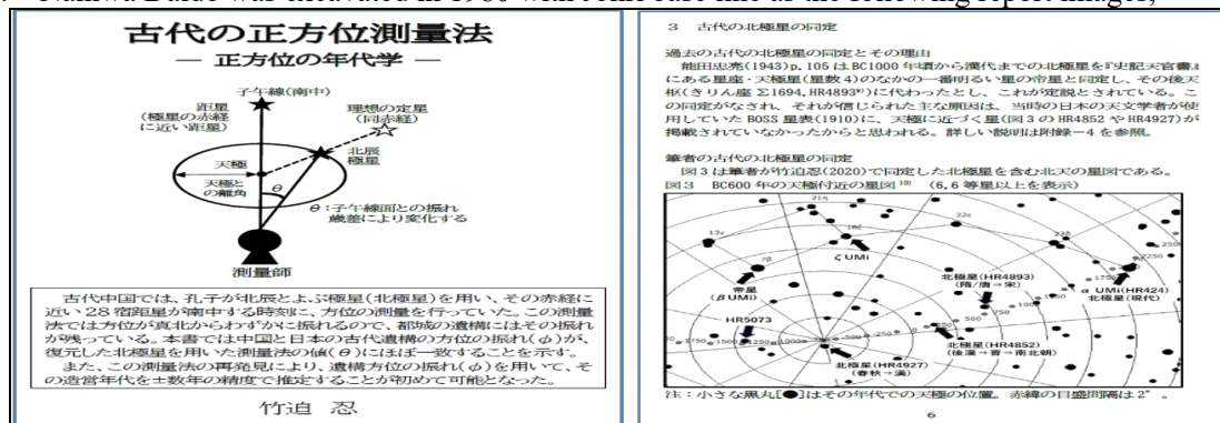
Figure 2-2-3-01 Shinobu Takesako : Identification of ancient pole star direction
