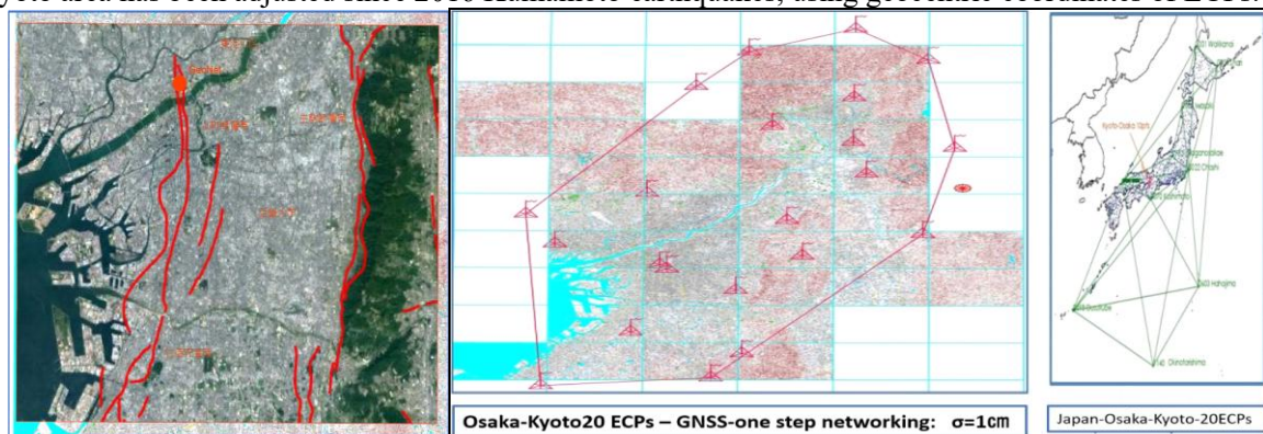
Figure 1-01: Osaka Uemachi and Ikoma active faults (AIST database)
