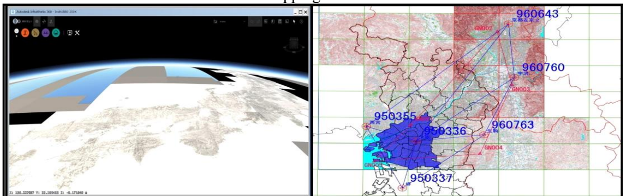
Figure 1: 1880s maps on CAD Globe : Osaka GNSS geodetic networking
