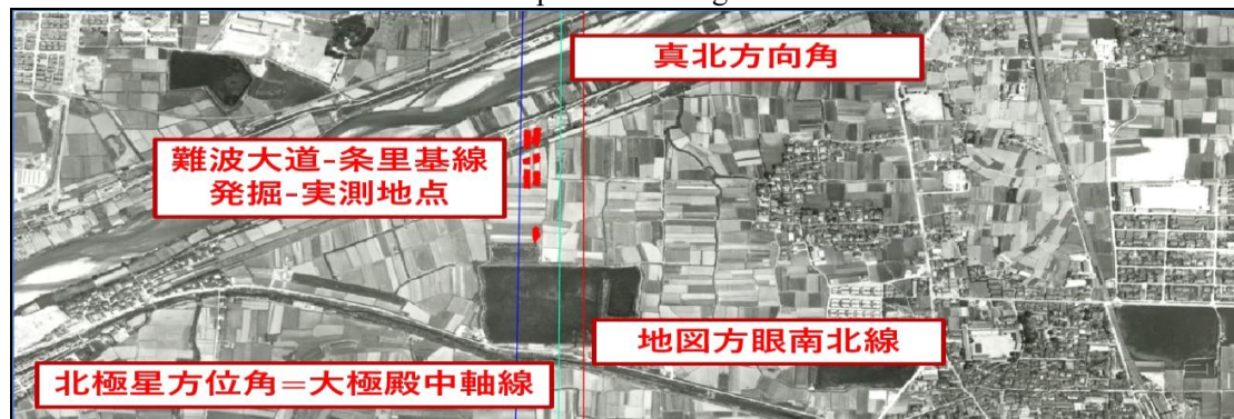
Figure 2-2-3-03: Coincidence among North Star Azimuth, excavated Johri base line on the 1961 ortho image
