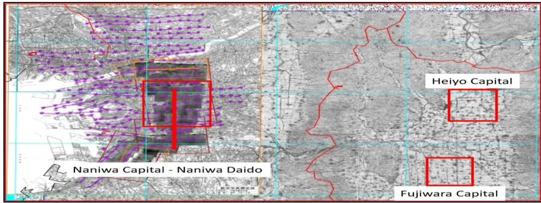
Figure 2-2-2-01: Naniwa Capital - Naniwa Daido, Fujiwara • Heiyo capitals
