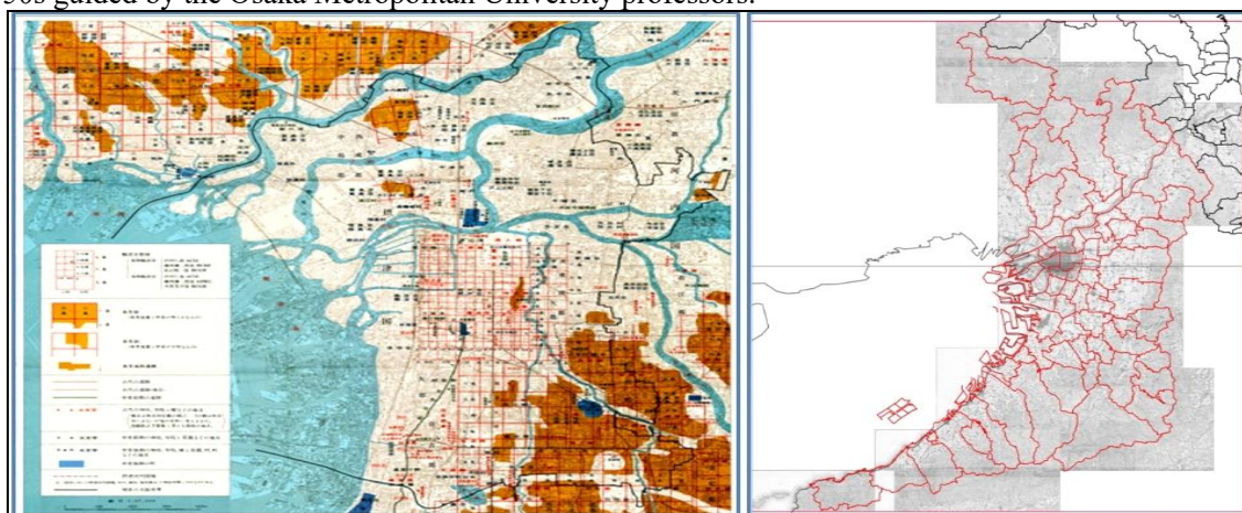
Figure 2-2-01: Osaka-Naniwa-capital and JohRi land administration (Osaka prefectural history (M. Hattori: OMU))
