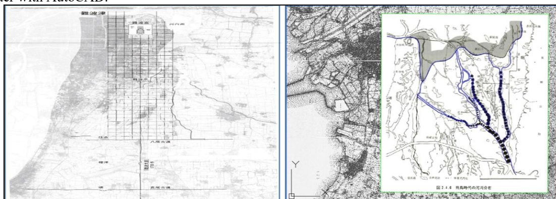
Figure 2-2-1-01: Replacement of the Yamato River in 1704 and the old channels
