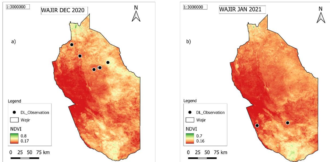
Fig 5: Wajir county ; desert locust observation in a) Dec 2020 and b) January 2021
