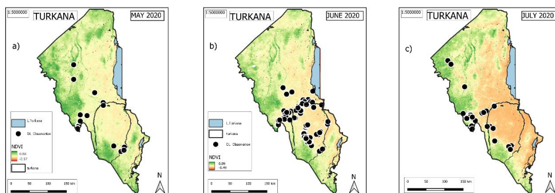
Fig 3: Turkana county; desert locust observation in the month of a) May, b) June and c) July
