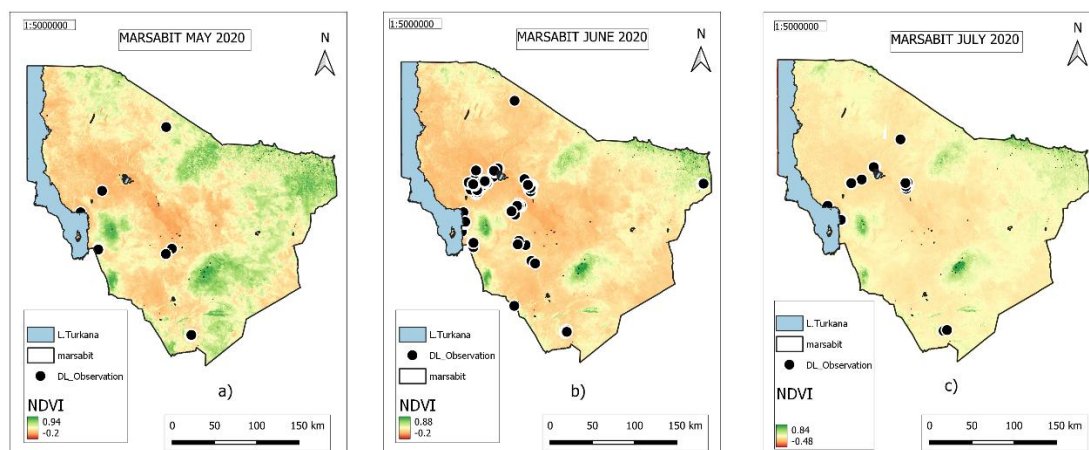
Fig 4: Mandera county; desert locust observation in the month of a) May, b) June and c) July 2020
