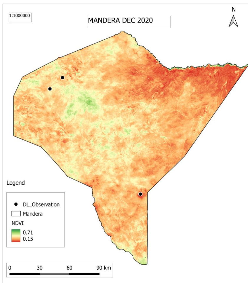
Fig 6: Desert Locust observation in Manderla county in December 2020
