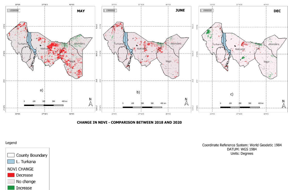
Fig 7: Comparison of vegetation loss between 2018 and 2020 in the months of May, June and December.
