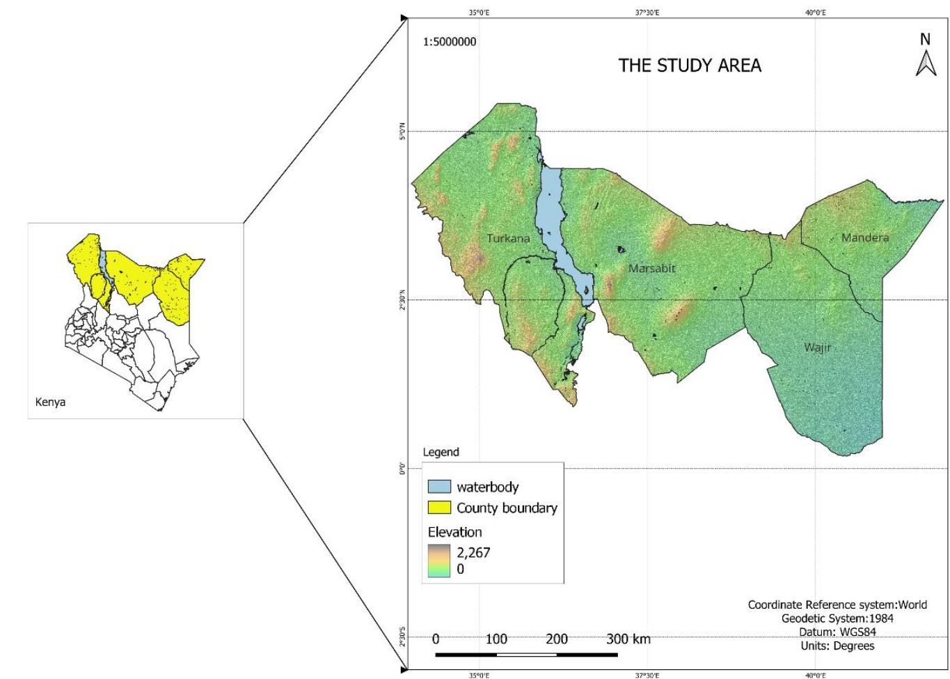
Figure 1: A map showing the study area (Turkana, Marsabit, Wajir and Mandera)
