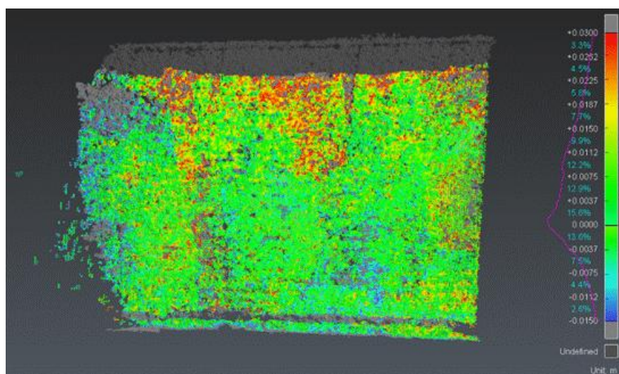
Figure 2: Cloud – Cloud Analysis Example
