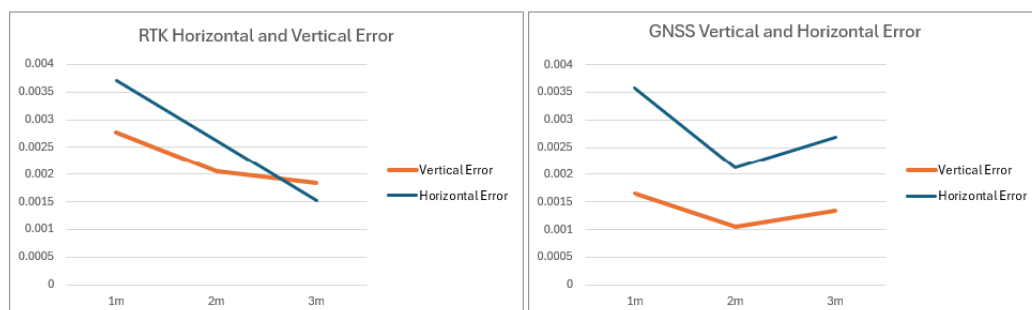
Figure 3 GNSS and RTK Horizontal vs Vertical Discrepancies
