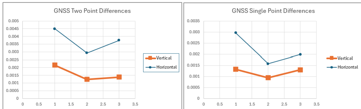
Figure 4 GNSS Two Point and Single Point Differences Horizontal Vs Vertical
