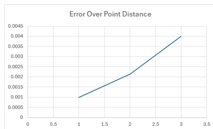
Figure 5 Error Over Point Distance GNSS
