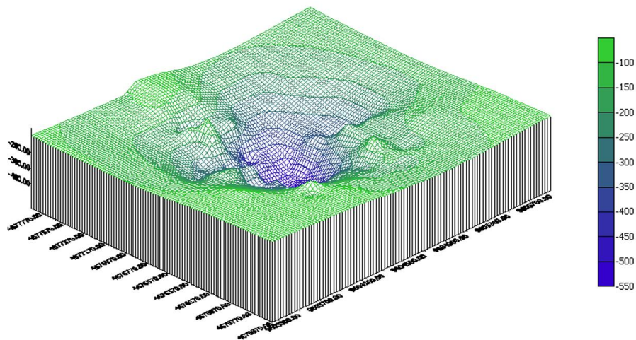
Figure 3. 3D image of the subsidence of the earth's surface (Valev et. al., 2015)
