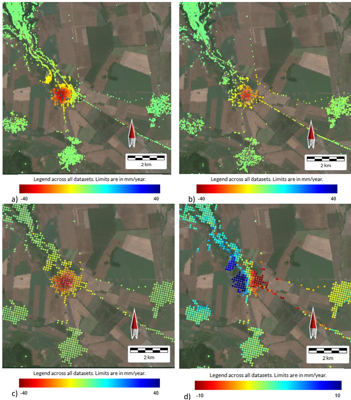
Figure 5. Mean LOS velocity (mm/yr) and time series Jan 2019-Dec2023 for the a) ascending 58 and 131 and b) descending orbits orbits 36 and 109 calibrated EGMS;
